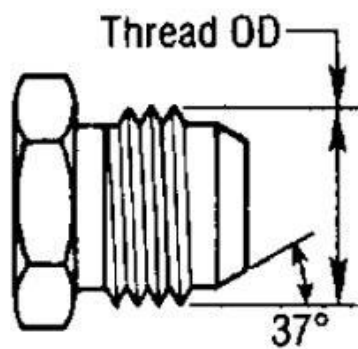
JIC 37° Male
